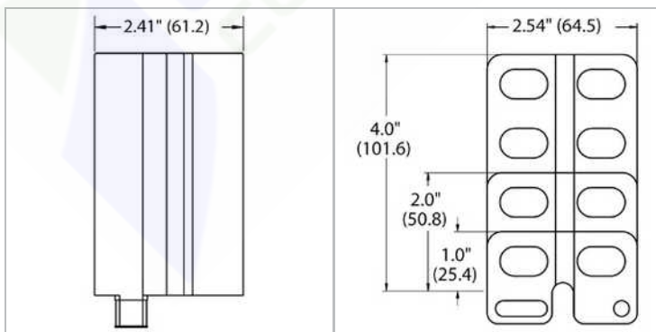
Side guards Side guards are available in 1/2\", 1\", 2\" and 4\" heights
